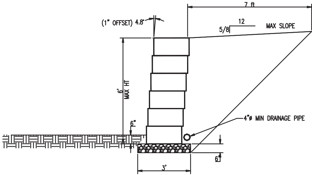
NO SOIL REINFORCEMENT USED
